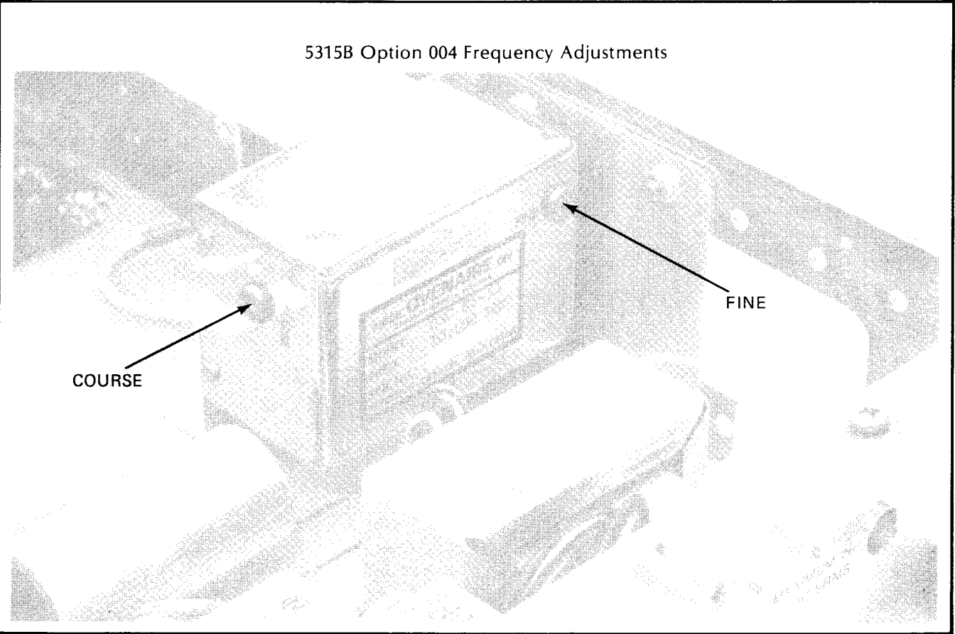
Figure 5-3. Reference Oscillator Adjustment Locations (Option 004)
