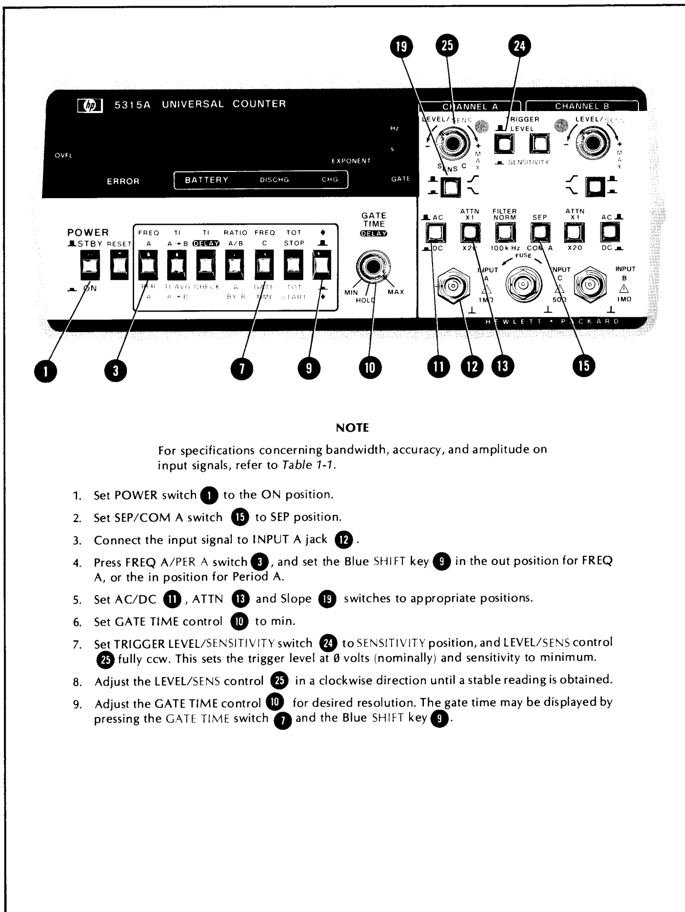
Figure 3-13. Frequency A/Period A Measurements
