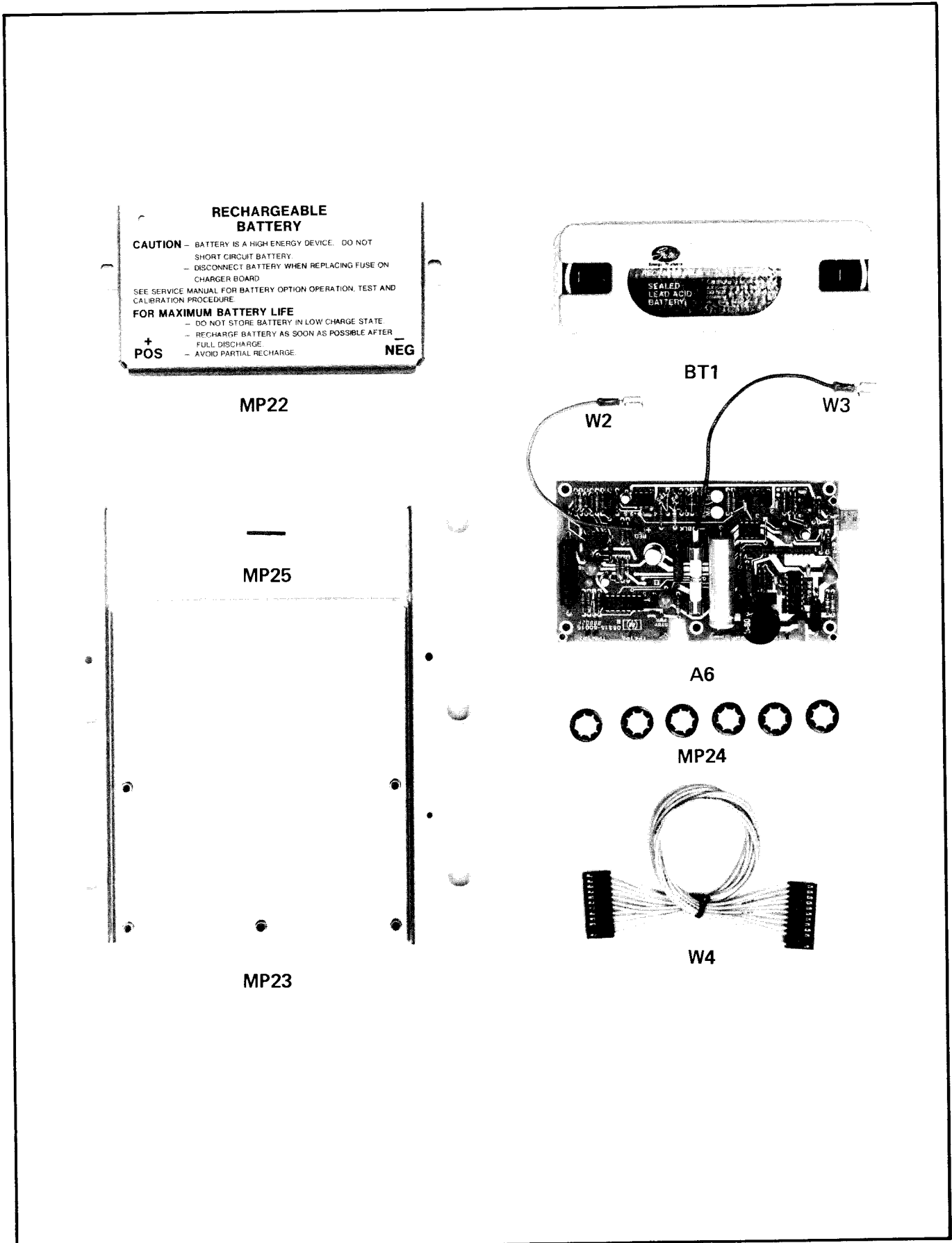
Figure 6-3. Option 002 Rechargeable Battery
